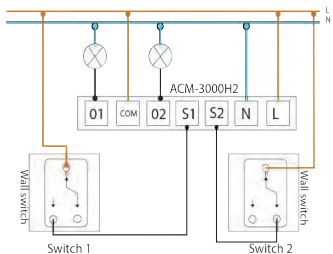
Technical installation schematic of the ACM-3000H2 with two wall switches (1 Corridor/Stairwell two-way switch)
