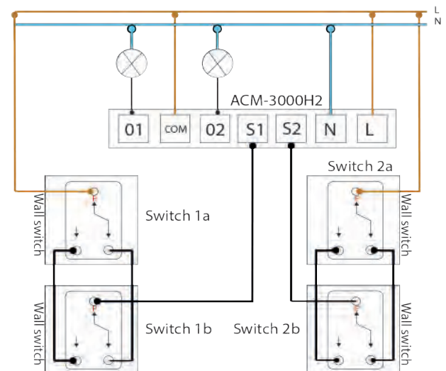
Technical installation schematic of the ACM-3000H2 with four wall switches (2 Corridor/Stairwell two-way switch)
