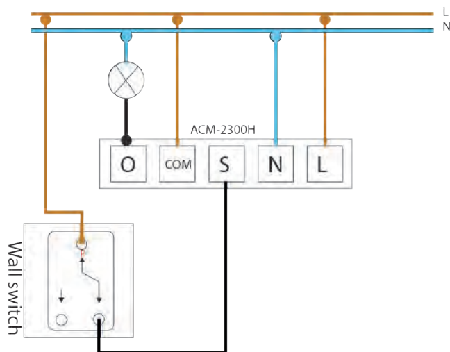
Technical installation schematic of the ACM-2300H with one wall switch.
