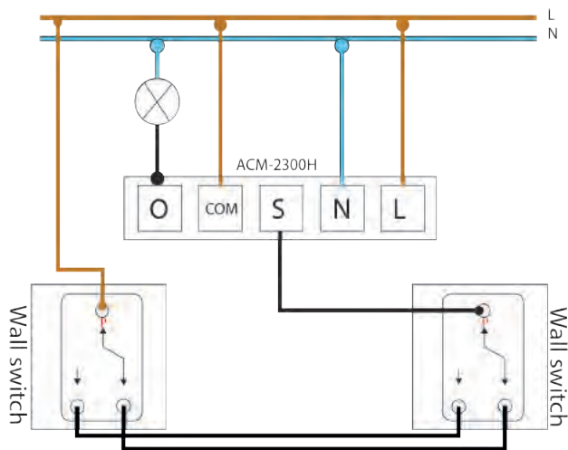
Technical installation schematic of the ACM-2300H with two wall switches (Corridor/Stairwell two-way switch)
